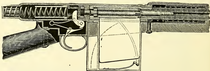
The Griffiths and Woodgate Automatic Rifle.
